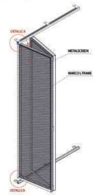
FOLDING L FRAME - METALSCREEN
